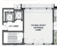
LOBBY KEY PLAN (GROUND FLOOR)
