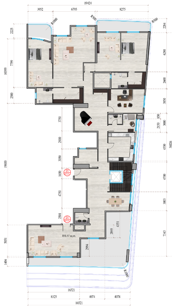
1 49th FLOOR PLAN DUPLEX 1 - LOWER FLOOR
