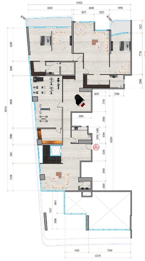
2 46th FLOOR PLAN DUPLEX 2 - UPPER FLOOR
