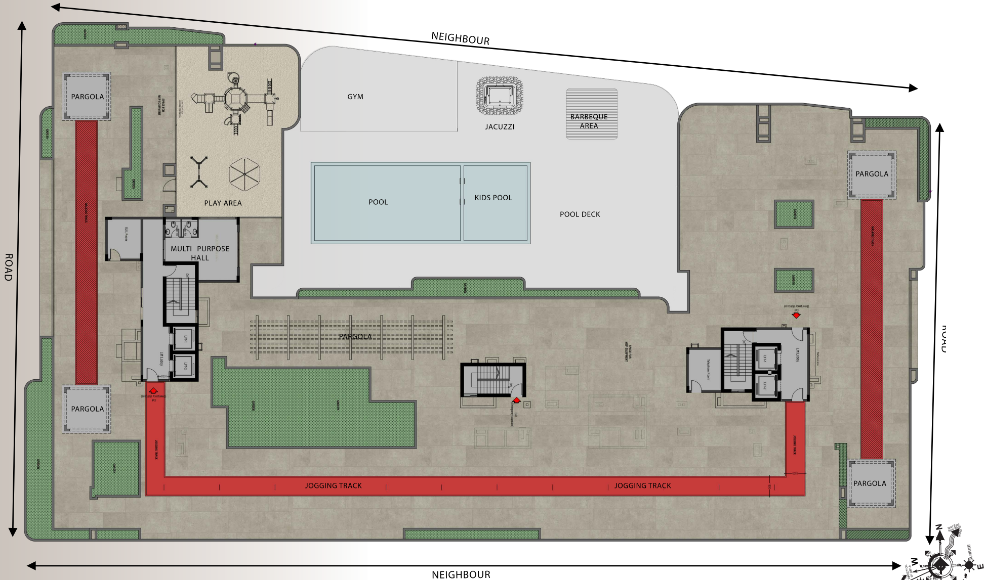
ROOF LAYOUT
