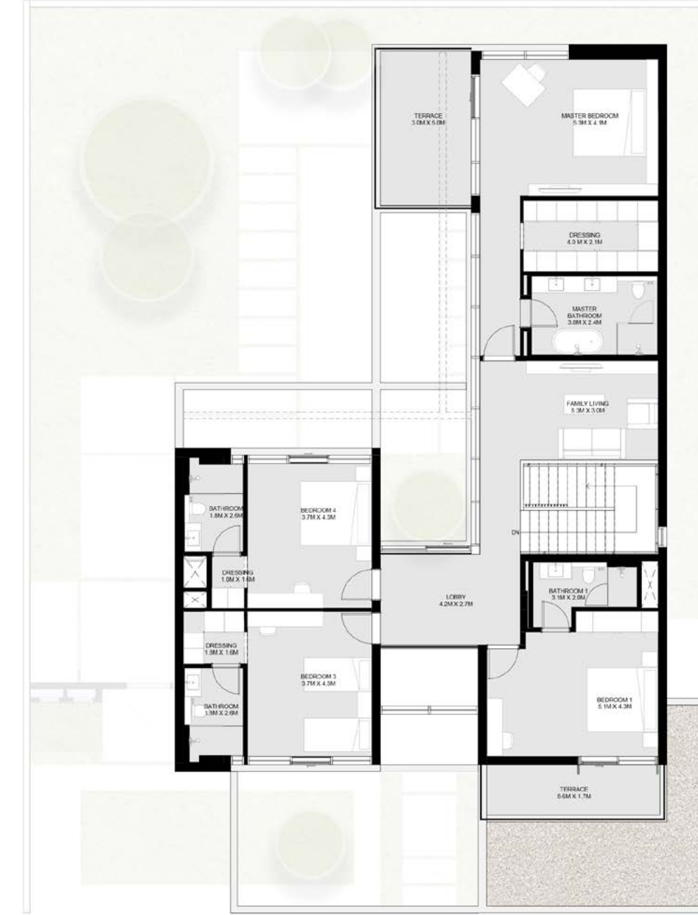
First Floor
