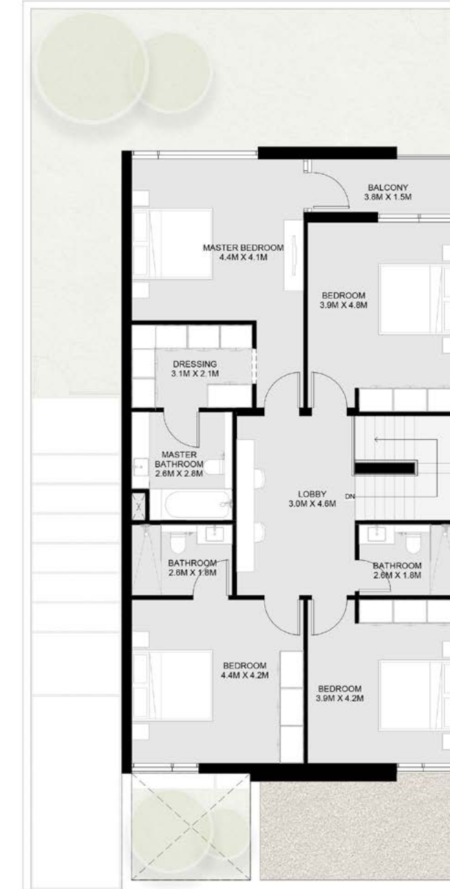
First Floor
