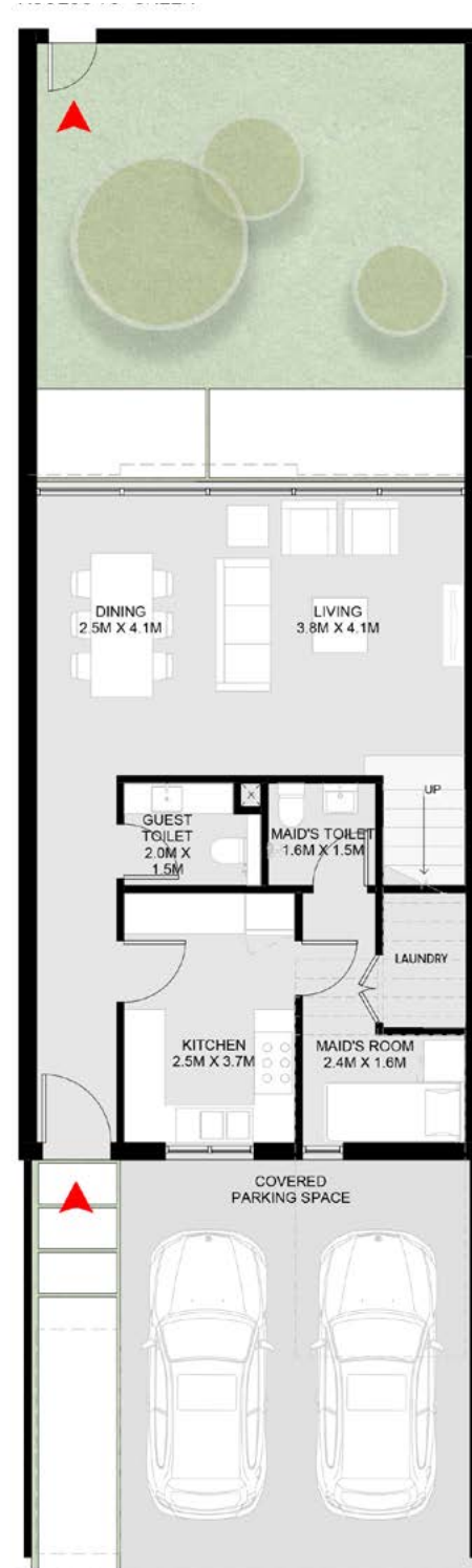
Ground Floor
