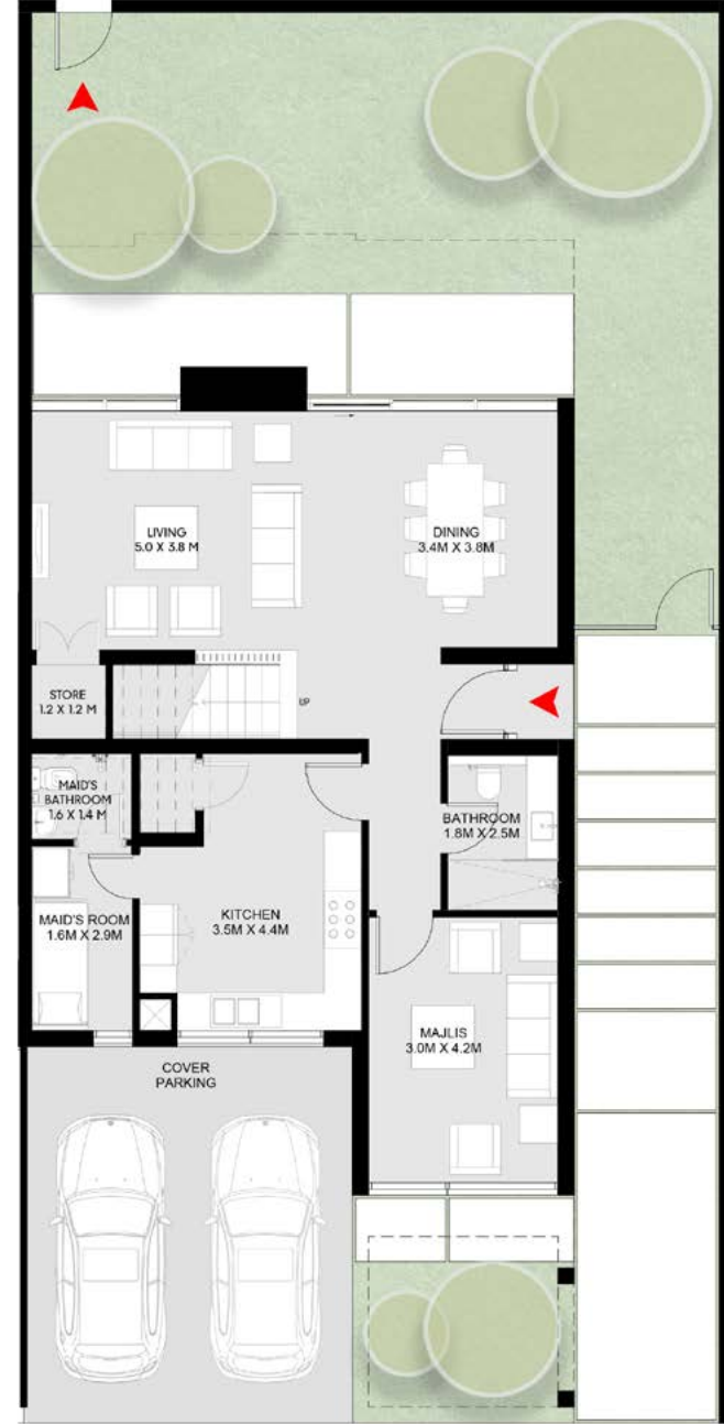
Ground Floor
