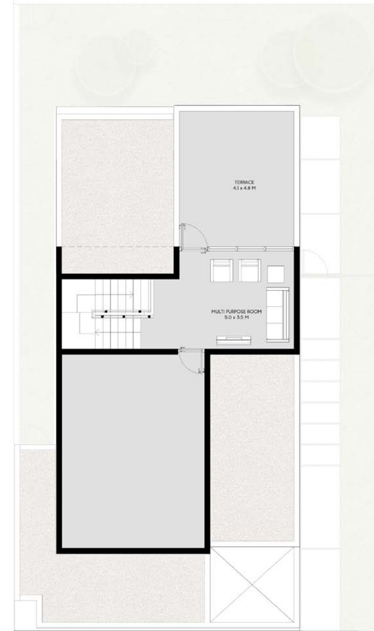
Second Floor
