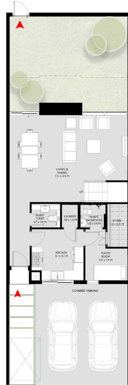
Ground Floor
